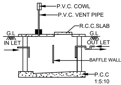
SEC. OF SEPTIC TANK
