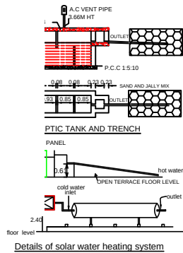
Details of solar water heating system
