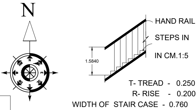
DETAILS OF STAIRCASE
