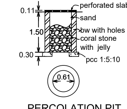
PERCOLATION PIT
