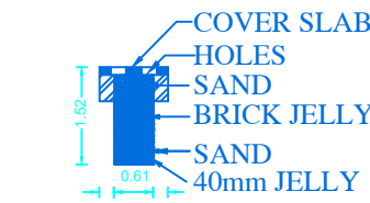
SECTION OF RAIN WATER COLLECTION TANK
