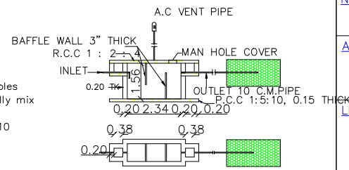
SEPTIC TANK & TRENCH
