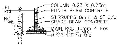
TYPICAL SECTION OF R.C.C. COLUMN FOUNDATION
