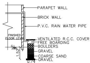
RAIN WATER HARVESTING (RWH) SYSTEM
