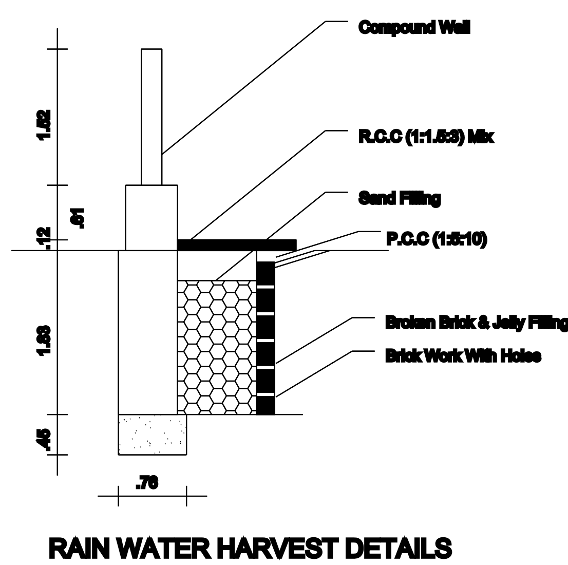
RAIN WATER HARVEST DETAILS
