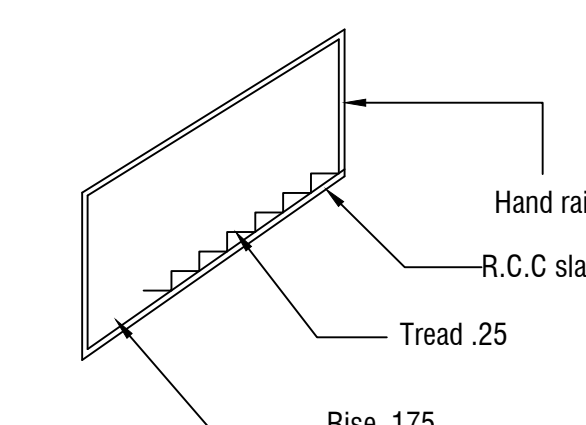
STAIR DETAIL
