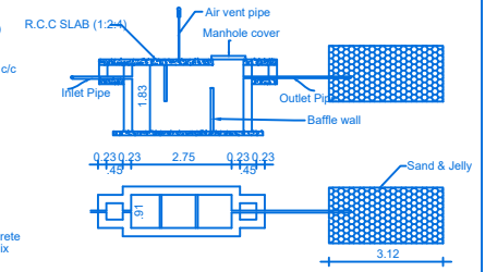
SEPTIC TANK & TRENCH
