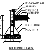
Column Details
