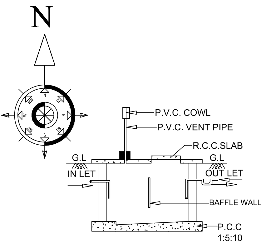
SEC. OF SEPTIC TANK
