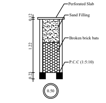
DRAINAGE SOAK PIT DETAILS
