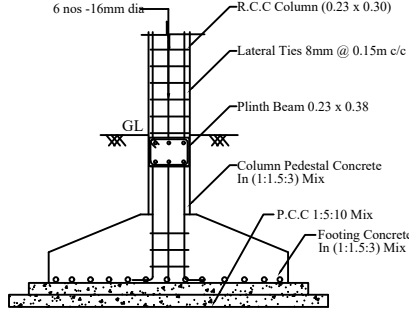
COLUMN FOOTING DETAILS
