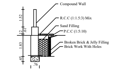
RAIN WATER HARVEST DETAILS
