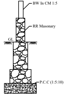
DETAILS OF RR MASONARY
