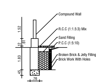
RAIN WATER HARVEST DETAILS
