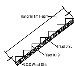
STAIR DETAILS
