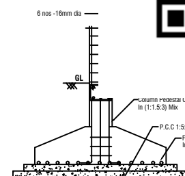
COLUMN FOOTING DETAILS
