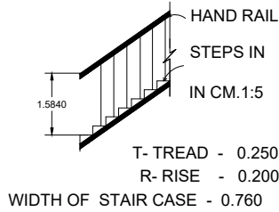
DETAILS OF STAIRCASE
