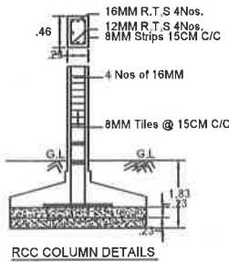
RCC COLUMN DETAILS
