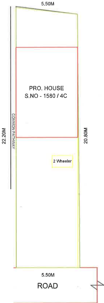
SITE PLAN
