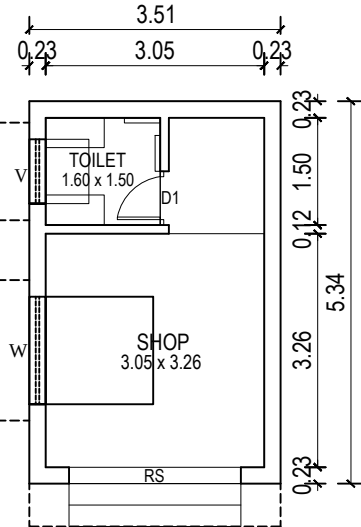
GF PLAN
