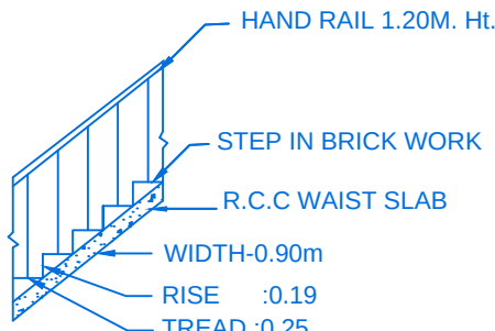
STAIR DETAIL
