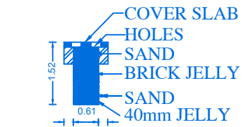
SECTION OF RAIN WATER COLLECTION TANK
