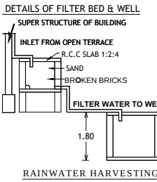
DETAILS OF FILTER BED & WELL
