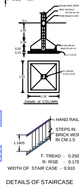
DETAILS OF STAIRCASE
