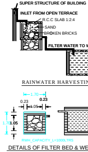
DETAILS OF FILTER BED & WELL
