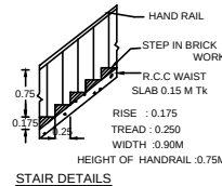
STAIR DETAILS
