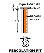
PERCOLATION PIT
