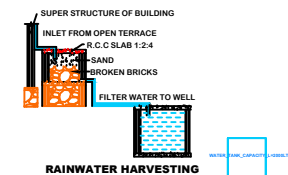
PERCOLATION PIT
