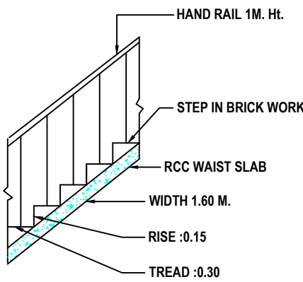
STAIR DETAIL
