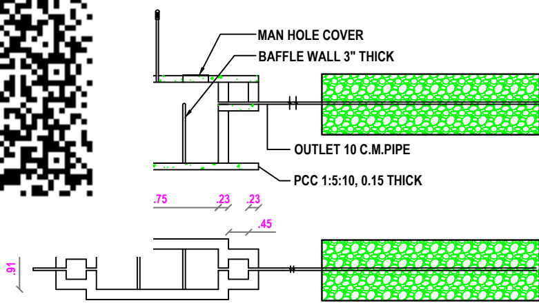
SEPTIC TANK & TRENCH
