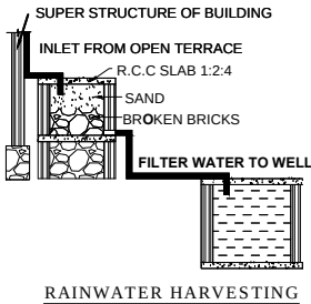
RAINWATER HARVESTING
