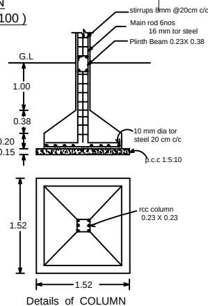
Details of COLUMN
