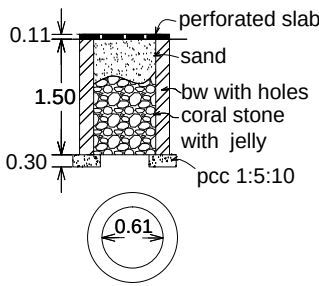
percolation pit
