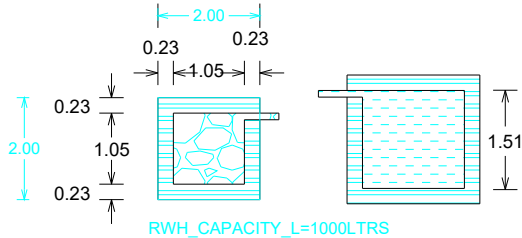
DETAILS OF FILTER BED & WELL
