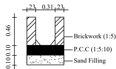
DETAILS OF DRAINAGE PIT
