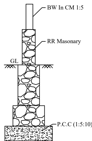
DETAILS OF RR MASONRY
