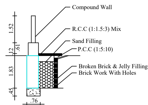
RAIN WATER HARVEST DETAILS
