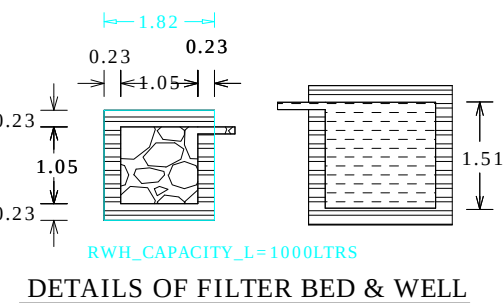
DETAILS OF FILTER BED & WELL
