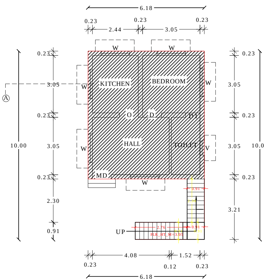
EXG.GROUND FLOOR PLAN
