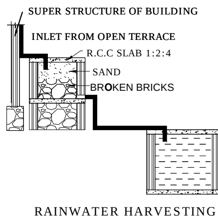
RAINWATER HARVESTING
