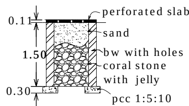
percolation pit
