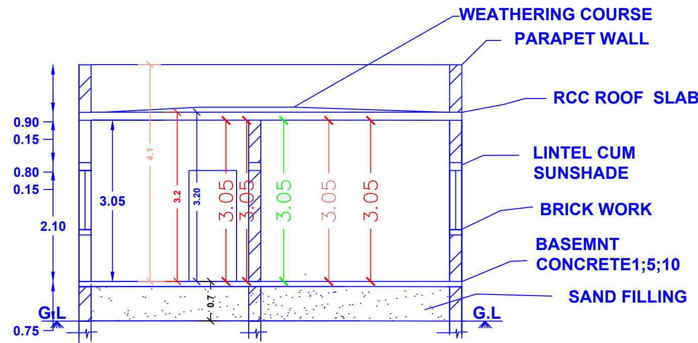
SECTION AB
