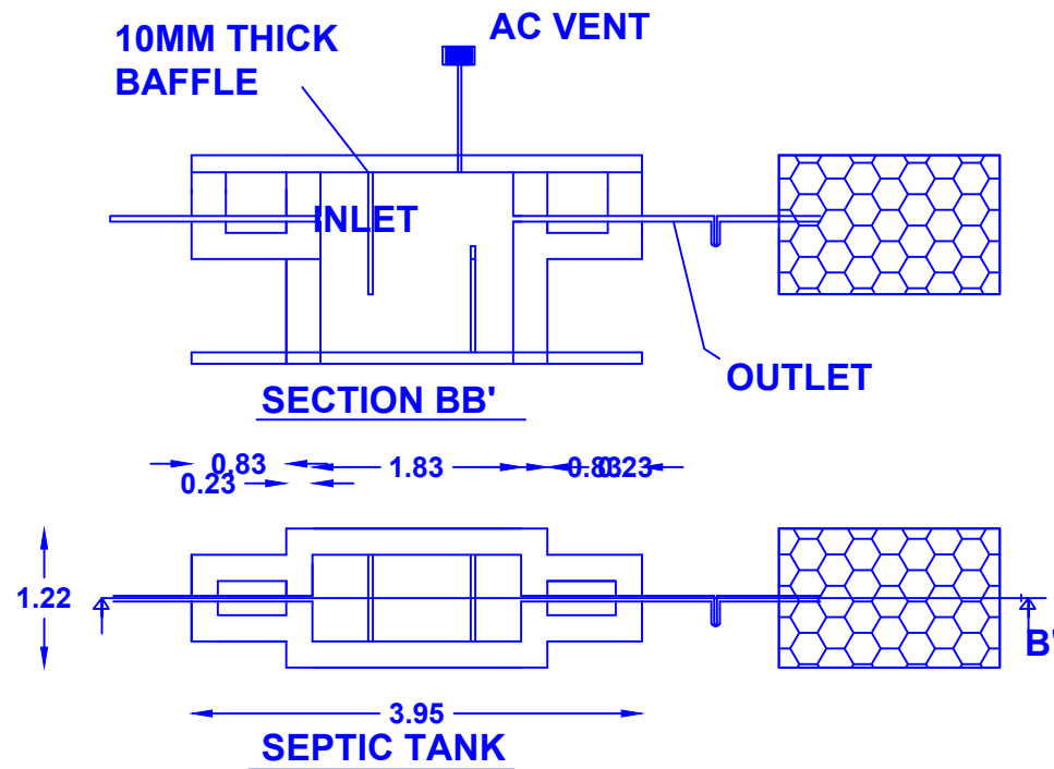
SECTION BB'
