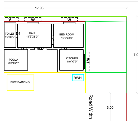
RESIDUARY SKETCH & SUPER IMPOSED SKETCH (SITE PLAN)
