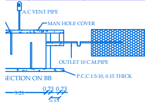
EXIS. SEPTIC TANK AND TRENCH & U TRAP ADOPTED
