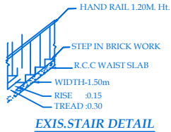
EXIS. STAIR DETAIL
