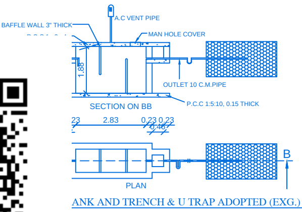
ANK AND TRENCH & U TRAP ADOPTED (EXG.)
