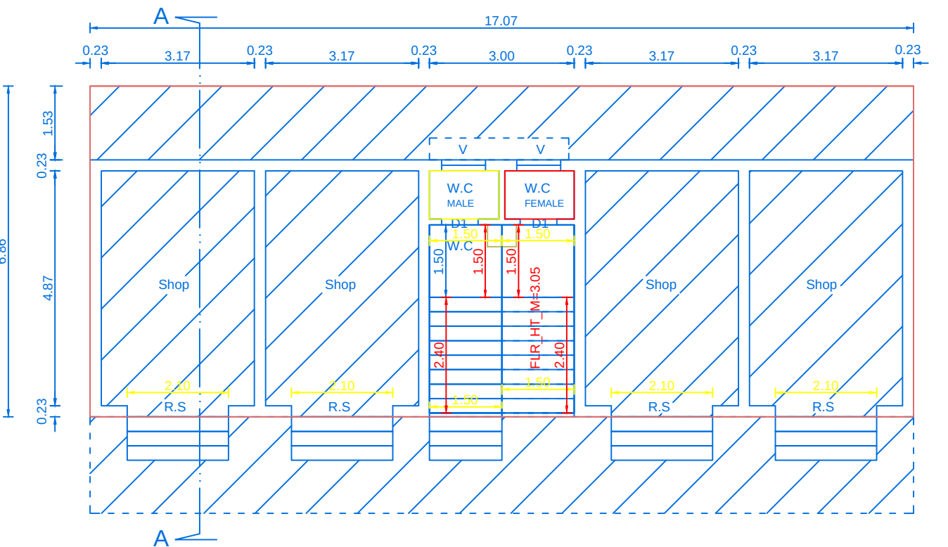
EXG.GROUND FLOOR
