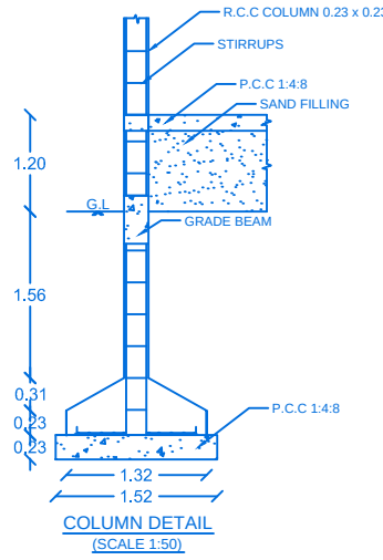
COLUMN DETAIL (SCALE 1:50)
