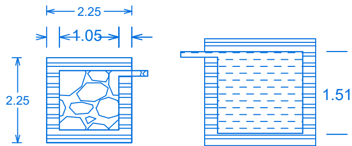
DETAILS OF FILTER BED & WELL
