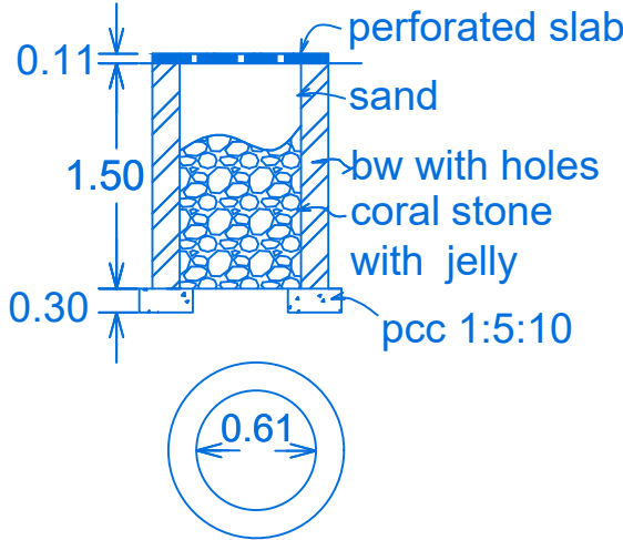
PERCOLATION PIT
