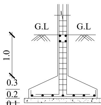
COLUMN FOOTING DETAILS - N.T.S
