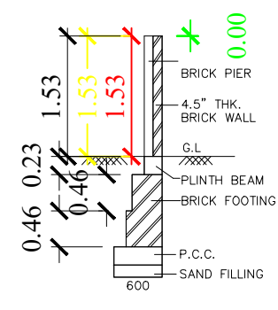
COMPOUND WALL DETAILS - N.T.S
