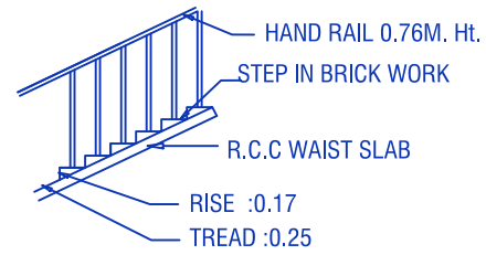
STAIR CASE DETAIL
