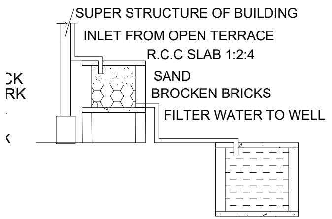
DETAILS OF FILTER BED & WELL
