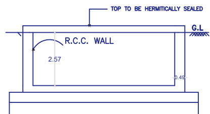
RWH SECTION (SAMPLE) RWH_CAPACITY_L=2000LTRS
