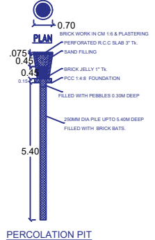
PERCOLATION PIT
