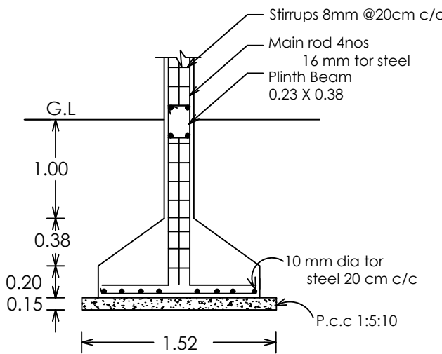
Details of column footing
