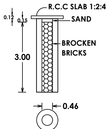
Percolation Pit
