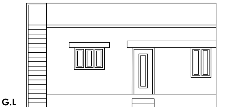
FRONT ELEVATION
