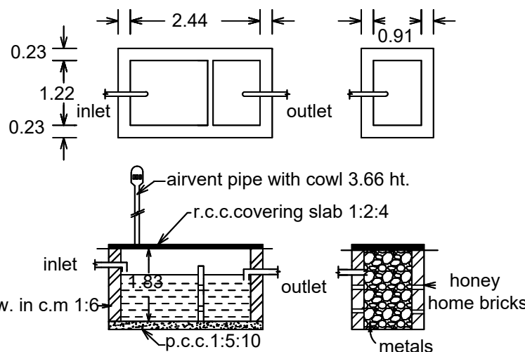
Details of septic tank and trench
