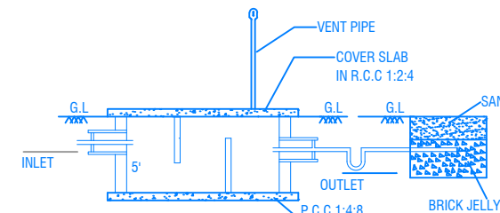
SECTION-A-B
