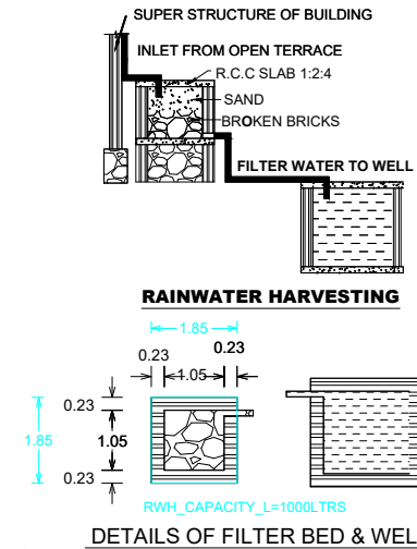
DETAILS OF FILTER BED & WELL
