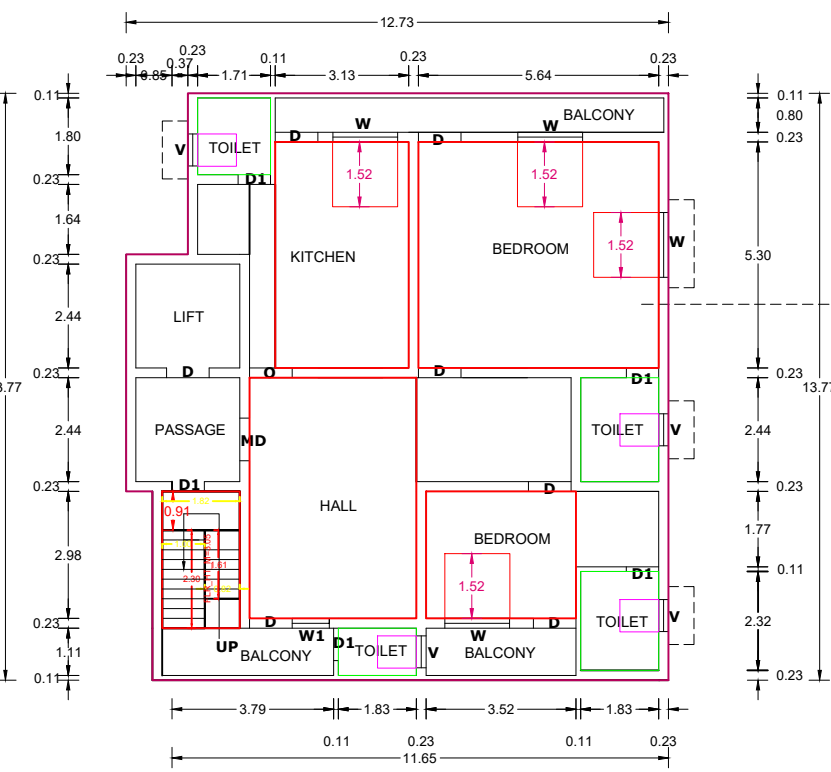
PRO.SECOND FLOOR PLAN
