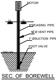
SEC. OF BOREWELL
