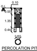
PERCOLATION PIT
