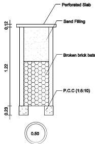
RAIN WATER COLLECTION WELL
