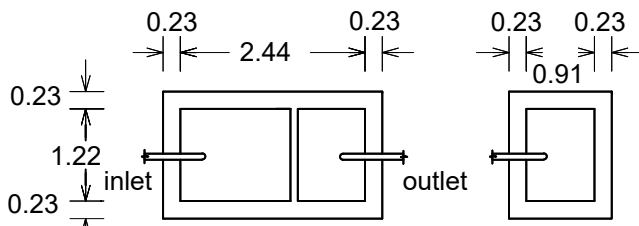
Details of rain water harvesting system
