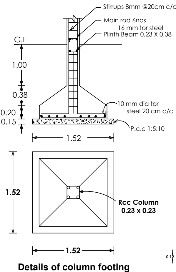
Details of column footing
