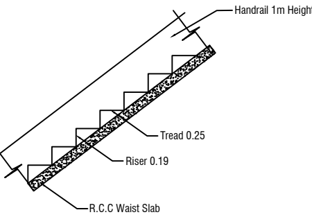
STAIR DETAILS
