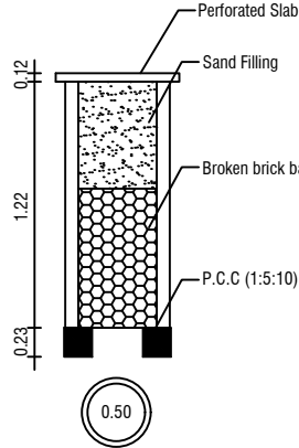
RAIN WATER COLLECTION WELL
