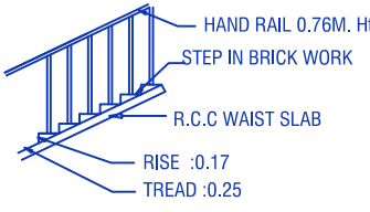
STAIR CASE DETAIL
