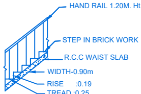
STAIR DETAIL
