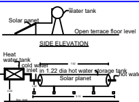
SOLAR WATER HEATER PLANT
