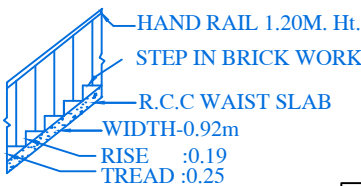
STAIR DETAIL
