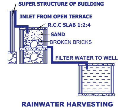
RAINWATER HARVESTING
