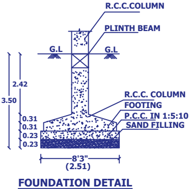
FOUNDATION DETAIL
