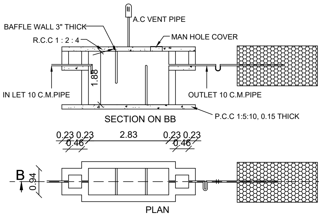
SEPTIC TANK AND TRENCH & U TRAP ADOPTED
