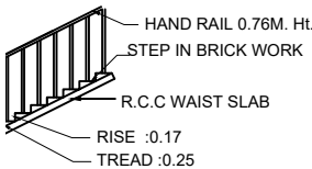
STAIR CASE DETAIL
